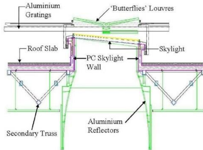
Figure 228: Cross Section Of Skylight At T3
