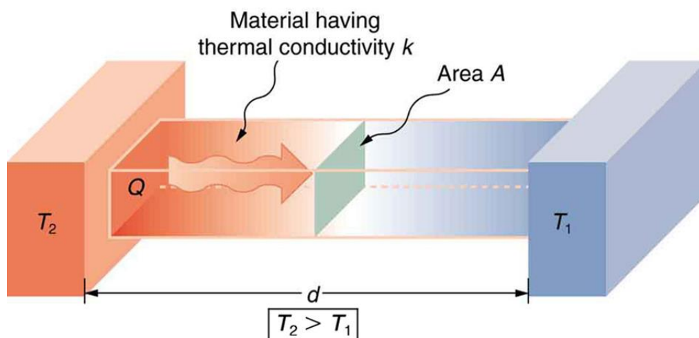
Figure 178: Heat Conduction Across Material (Image Credit: Openstax College Physics)
