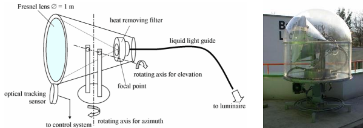
Figure 226: Fibre-Optic System
