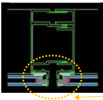
Figure 30 Typical Mullion
