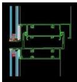
Figure 31 Typical Stack-Joint
