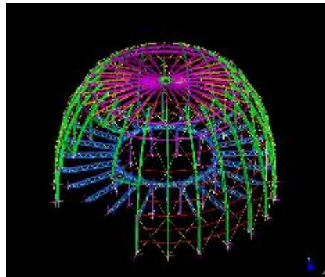
Figure 147: Structural Analysis
