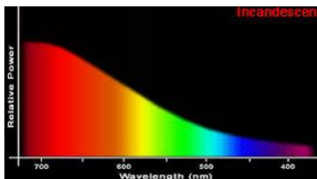
Figure 243: Full Spectrum Of An Incandescent / Halogen Lamp With CRI=100
