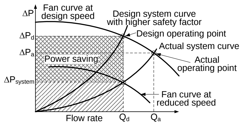
Figure 3.32 Fan performances due to use of high safety factors
